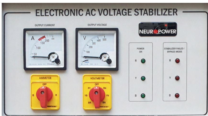
Control panel of AVS MCT
